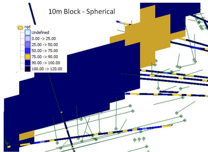
Figure 7. Comparison of interpolated RQD values in Model 2 and borehole RQD data
