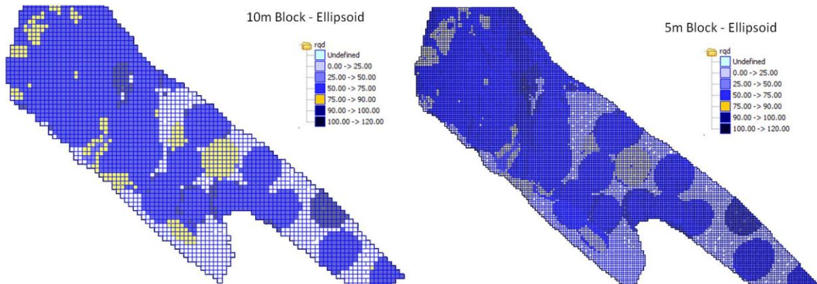
Figure 4. Comparison of interpolated RQD values in plan view between Model 1 using a 10m x 10m x 5m block size (left) and Model 3 using a 5m x 5m x 3m block size (right)
