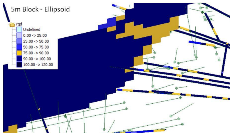
Figure 8. Comparison of interpolated RQD values in Model 3 and borehole RQD data
