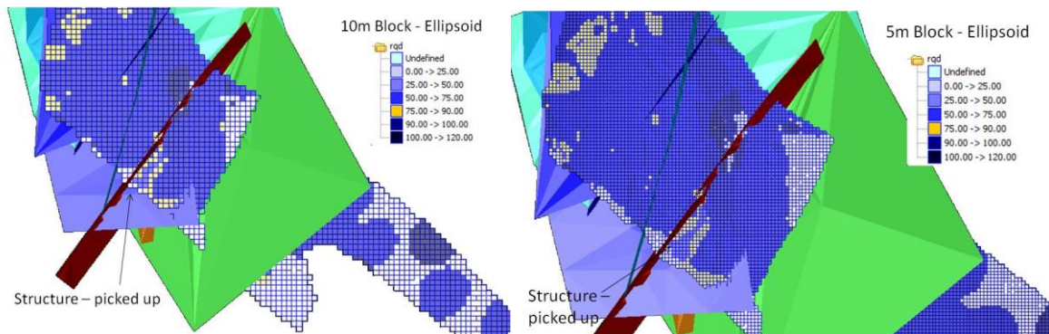
Figure 5. Pick up of a structure in Model 1 (left) and Model 3 (right)
