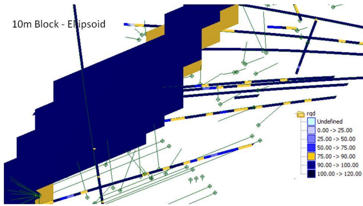
Figure 6. Comparison of interpolated RQD values in Model 1 and borehole RQD data
